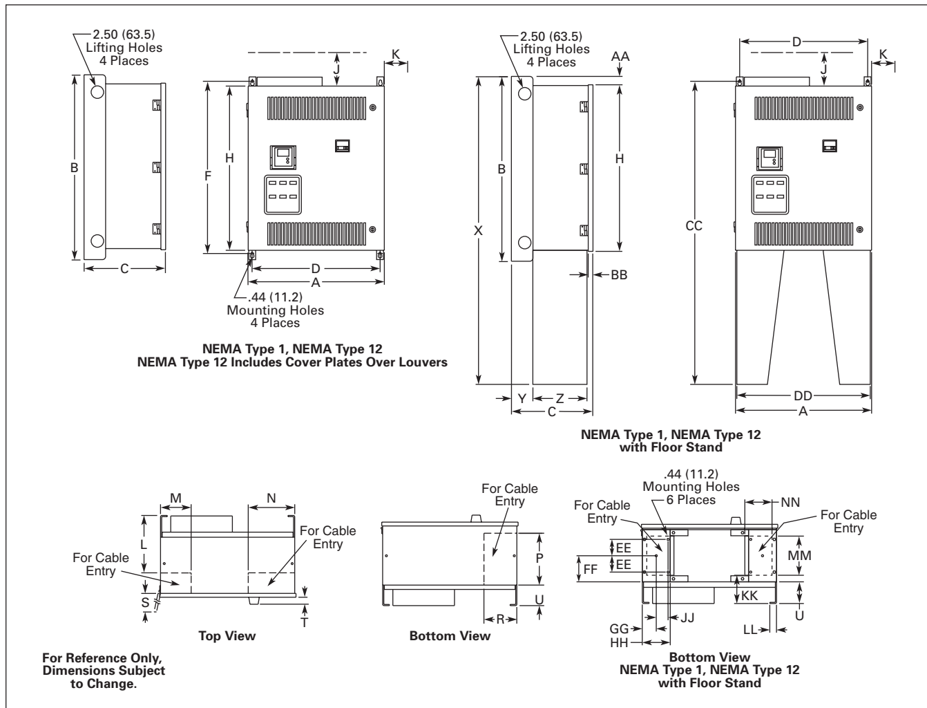
Figure 19. Approximate Dimensions
